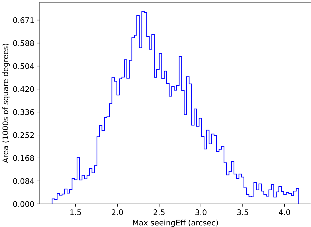
too_elab_r64_d2_griz_v3.4_10yrs All sky u band: Max seeingEff
