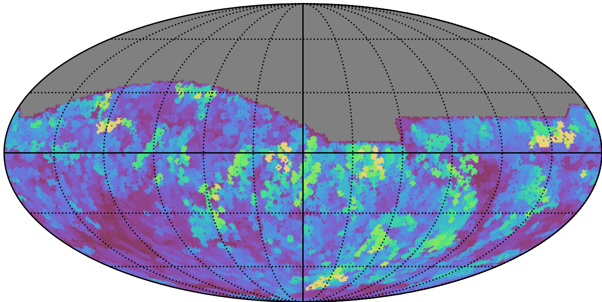
too_elab_r64_d2_griz_v3.4_10yrs All sky r band: Max seeingEff
