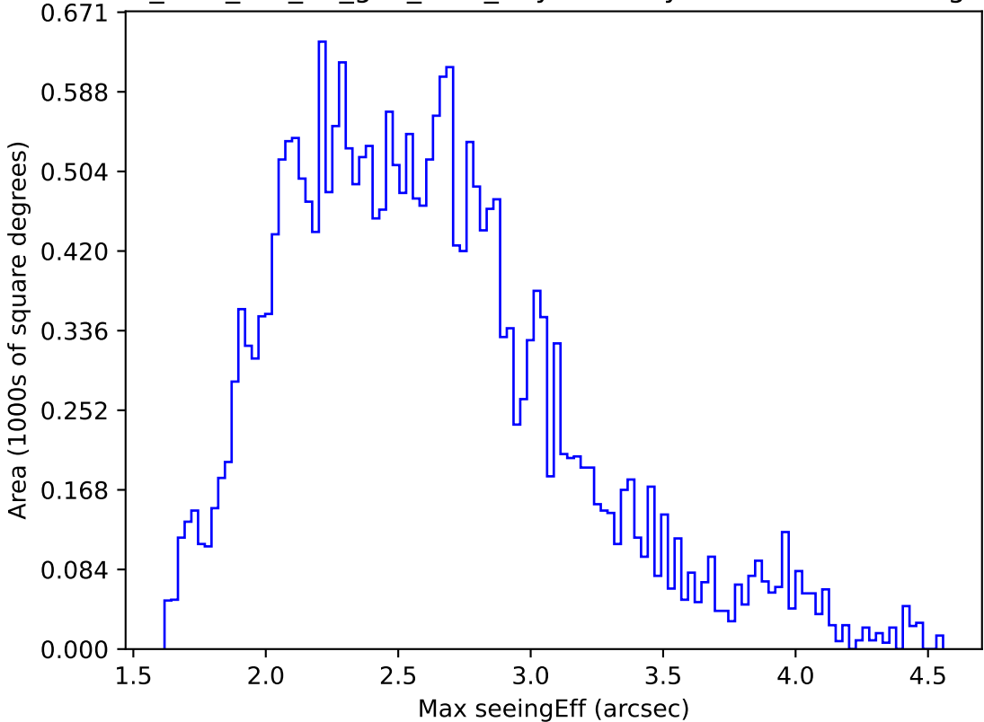
too_elab_r64_d2_griz_v3.4_10yrs All sky r band: Max seeingEff
