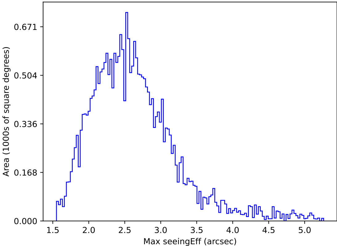
too_elab_r64_d2_griz_v3.4_10yrs All sky i band: Max seeingEff
