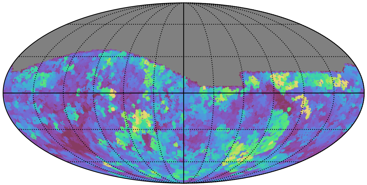
too_elab_r64_d2_griz_v3.4_10yrs All sky g band: Max seeingEff
