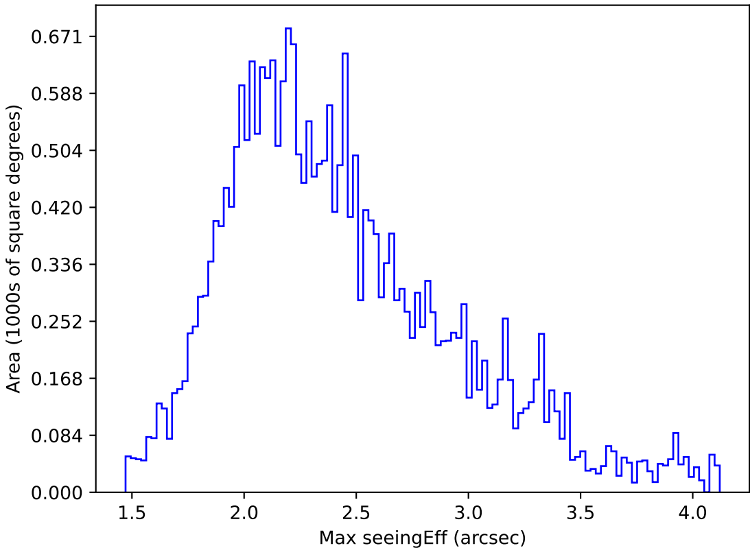
too_elab_r64_d2_griz_v3.4_10yrs All sky g band: Max seeingEff
