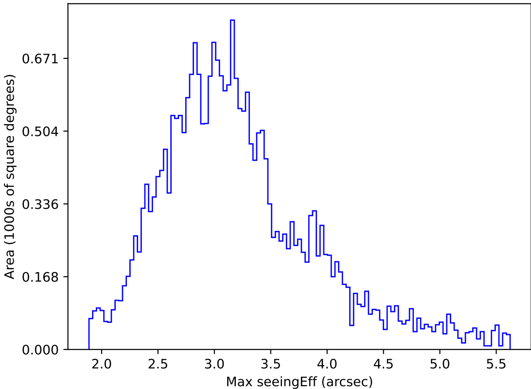
too_elab_r64_d2_griz_v3.4_10yrs All sky all bands: Max seeingEff
