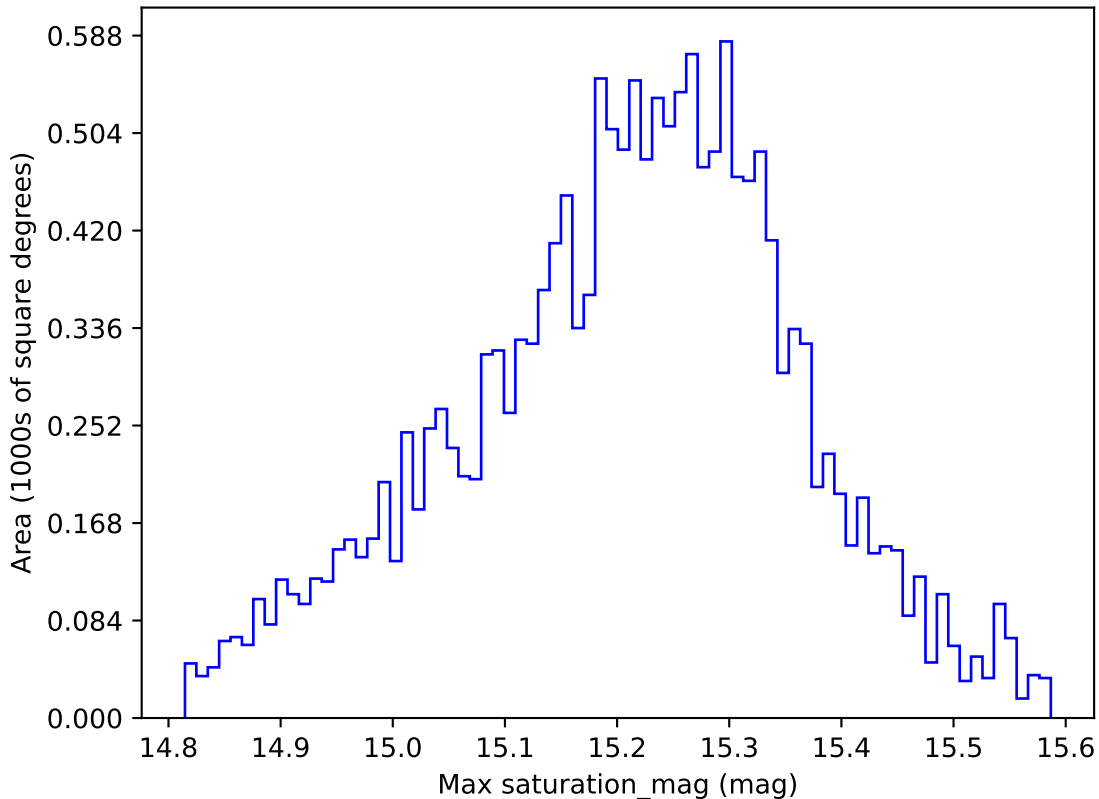
too_elab_r64_d2_griz_v3.4_10yrs WFD z band: Max saturation_mag
