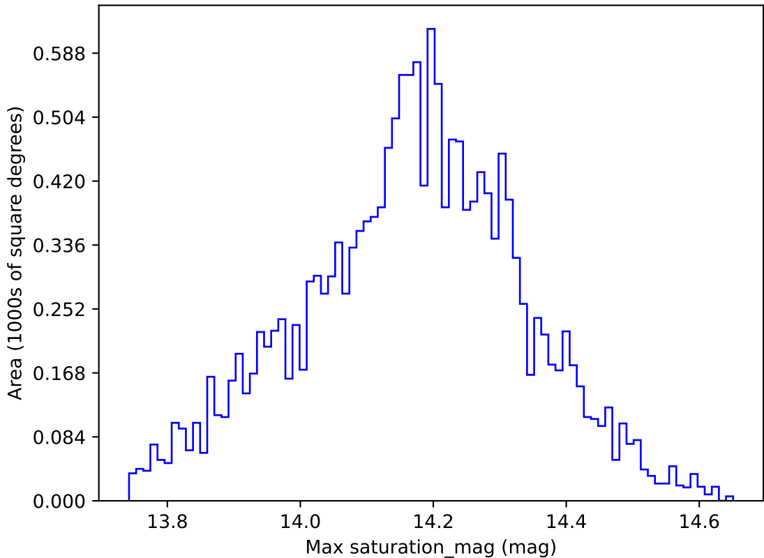
too_elab_r64_d2_griz_v3.4_10yrs WFD y band: Max saturation_mag
