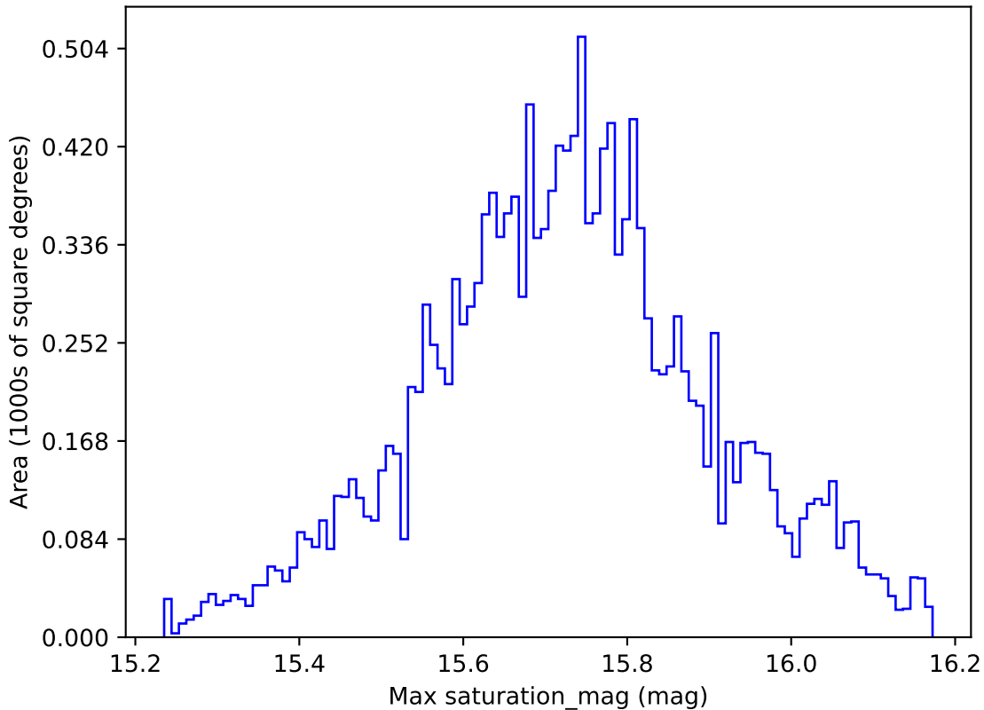
too_elab_r64_d2_griz_v3.4_10yrs WFD g band: Max saturation_mag
