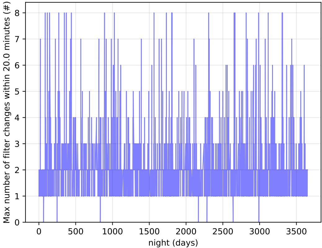
too_elab_r64_d2_griz_v3.4_10yrs Per Night: Max number of filter changes within 20.0 minutes
