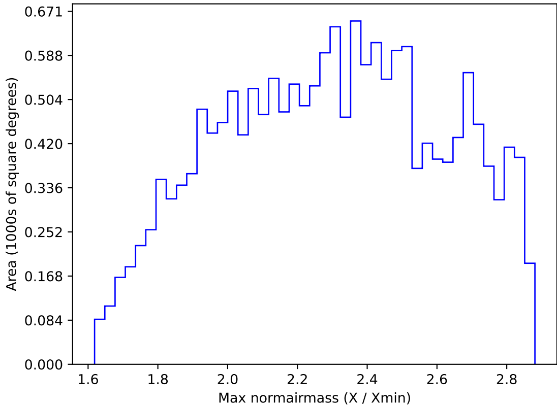
too_elab_r64_d2_griz_v3.4_10yrs WFD z band: Max normairmass
