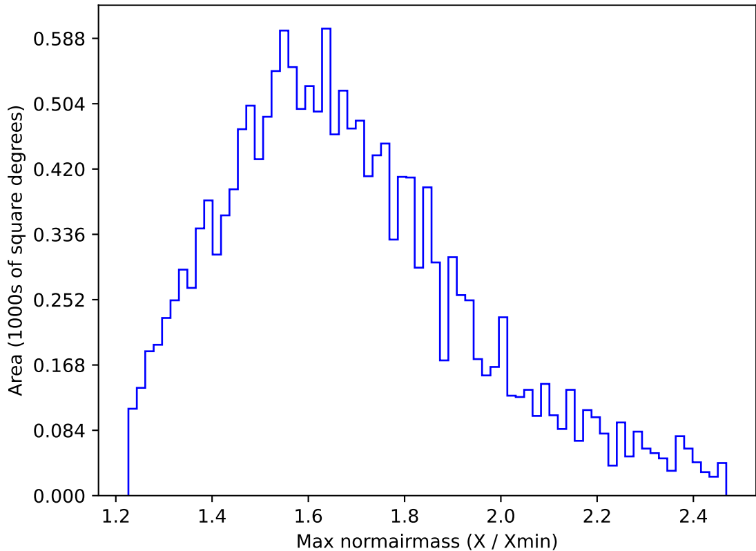
too_elab_r64_d2_griz_v3.4_10yrs WFD u band: Max normairmass
