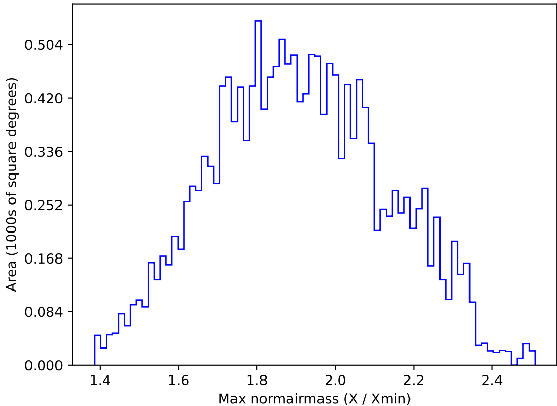
too_elab_r64_d2_griz_v3.4_10yrs WFD g band: Max normairmass
