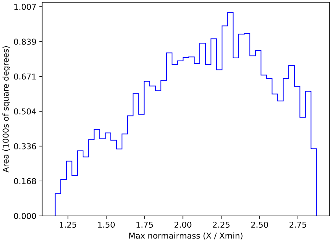
too_elab_r64_d2_griz_v3.4_10yrs All sky z band: Max normairmass
