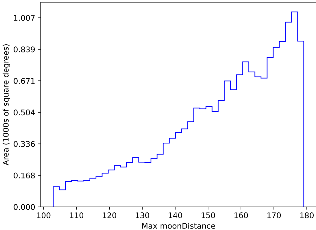
too_elab_r64_d2_griz_v3.4_10yrs WFD z band: Max moonDistance
