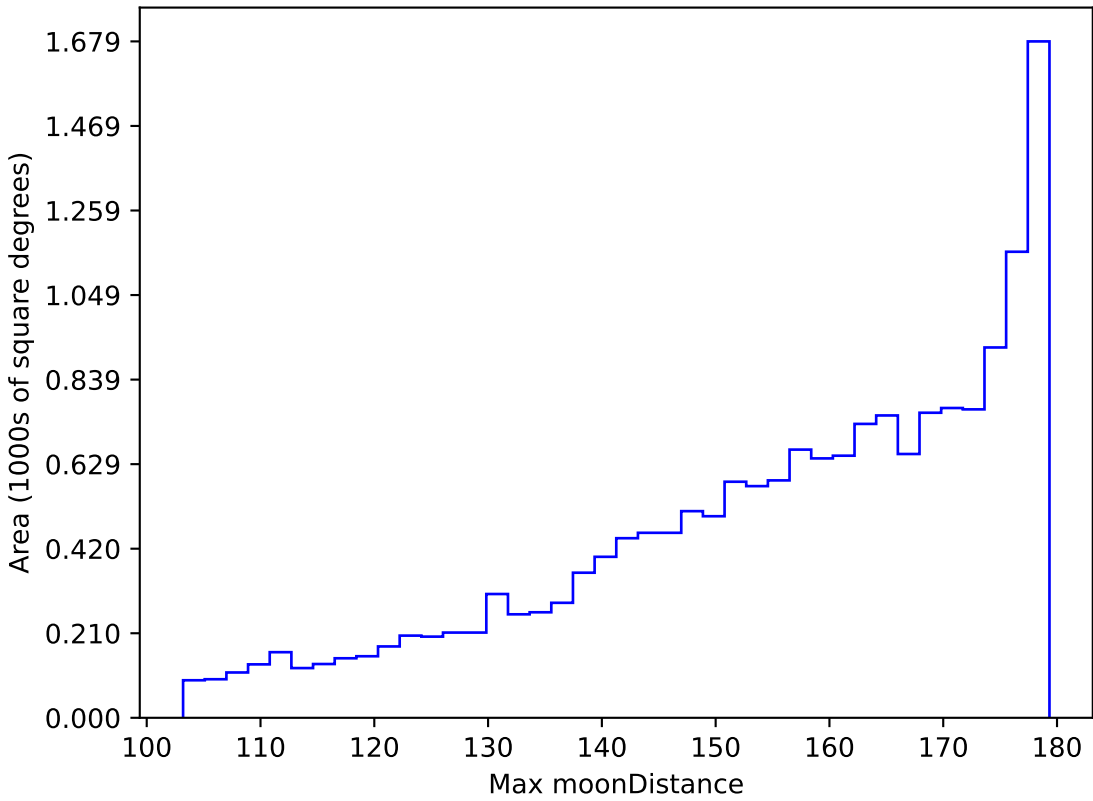
too_elab_r64_d2_griz_v3.4_10yrs WFD r band: Max moonDistance
