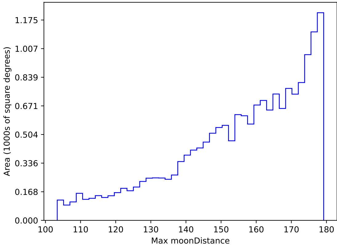
too_elab_r64_d2_griz_v3.4_10yrs WFD i band: Max moonDistance
