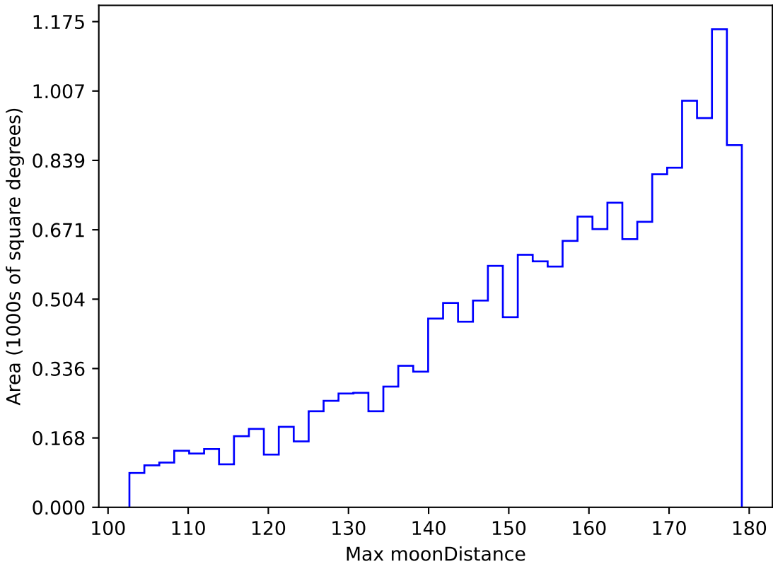
too_elab_r64_d2_griz_v3.4_10yrs WFD g band: Max moonDistance
