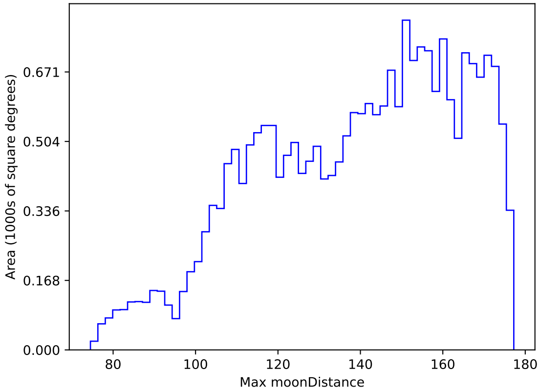
too_elab_r64_d2_griz_v3.4_10yrs All sky y band: Max moonDistance
