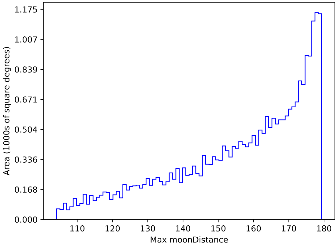
too_elab_r64_d2_griz_v3.4_10yrs All sky r band: Max moonDistance
