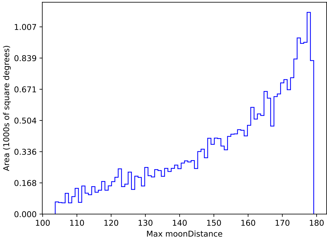
too_elab_r64_d2_griz_v3.4_10yrs All sky i band: Max moonDistance
