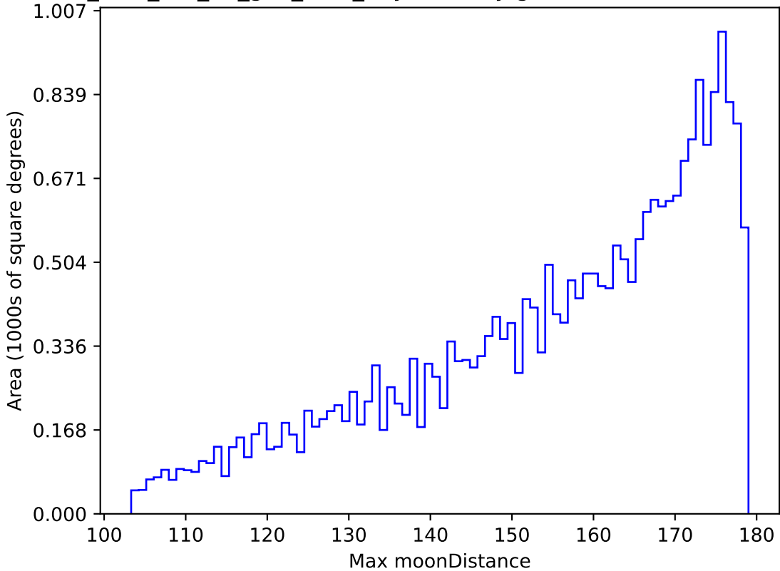
too_elab_r64_d2_griz_v3.4_10yrs All sky g band: Max moonDistance
