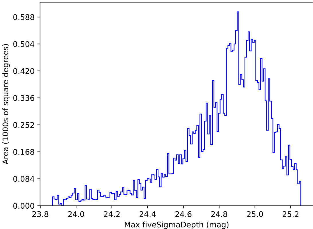
too_elab_r64_d2_griz_v3.4_10yrs Yr 1 g band: Max fiveSigmaDepth
