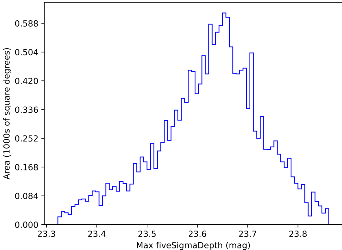
too_elab_r64_d2_griz_v3.4_10yrs WFD z band: Max fiveSigmaDepth
