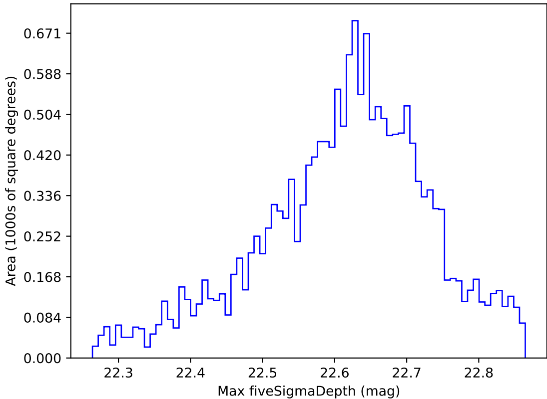
too_elab_r64_d2_griz_v3.4_10yrs WFD y band: Max fiveSigmaDepth
