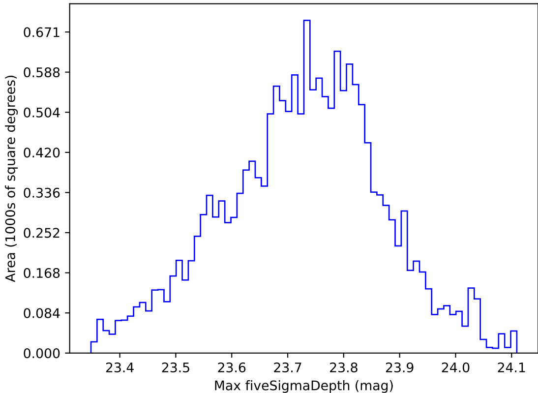
too_elab_r64_d2_griz_v3.4_10yrs WFD u band: Max fiveSigmaDepth
