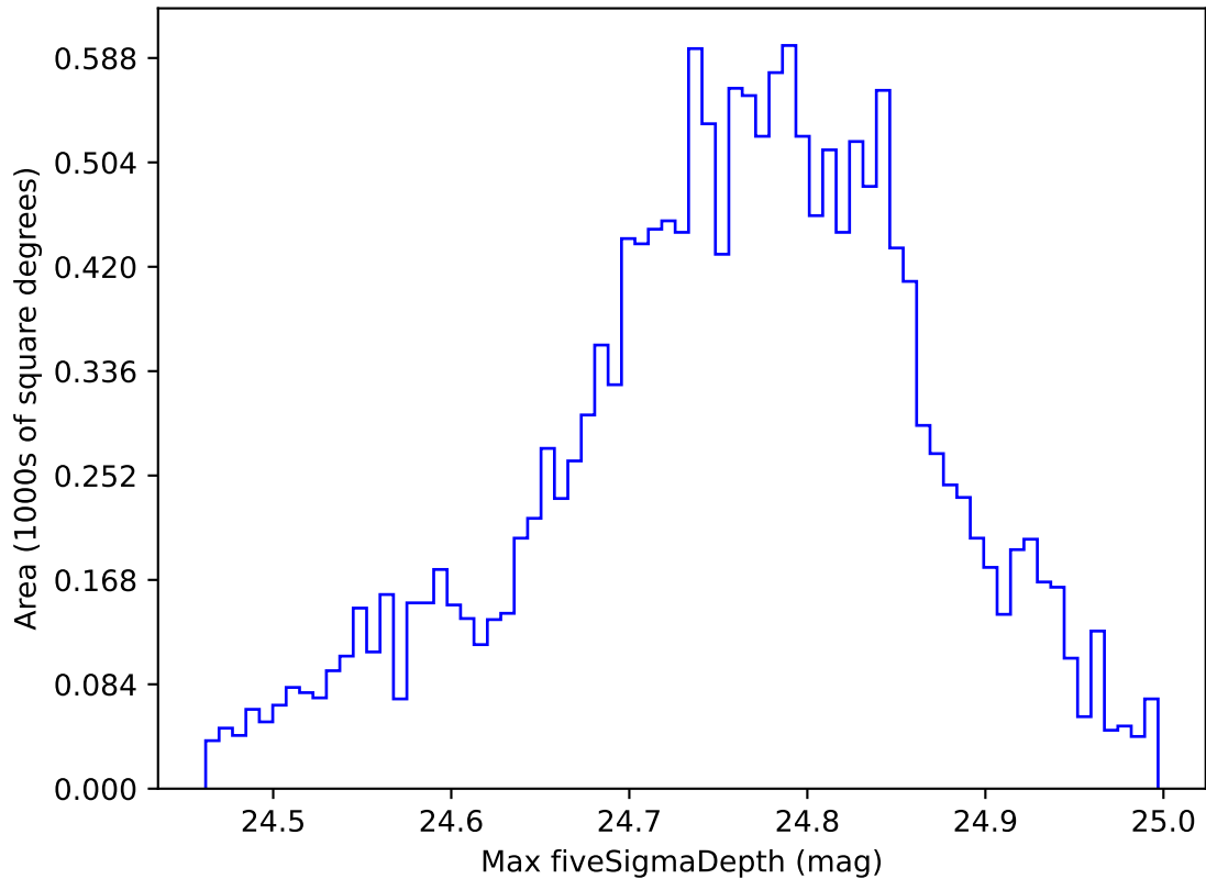
too_elab_r64_d2_griz_v3.4_10yrs WFD r band: Max fiveSigmaDepth
