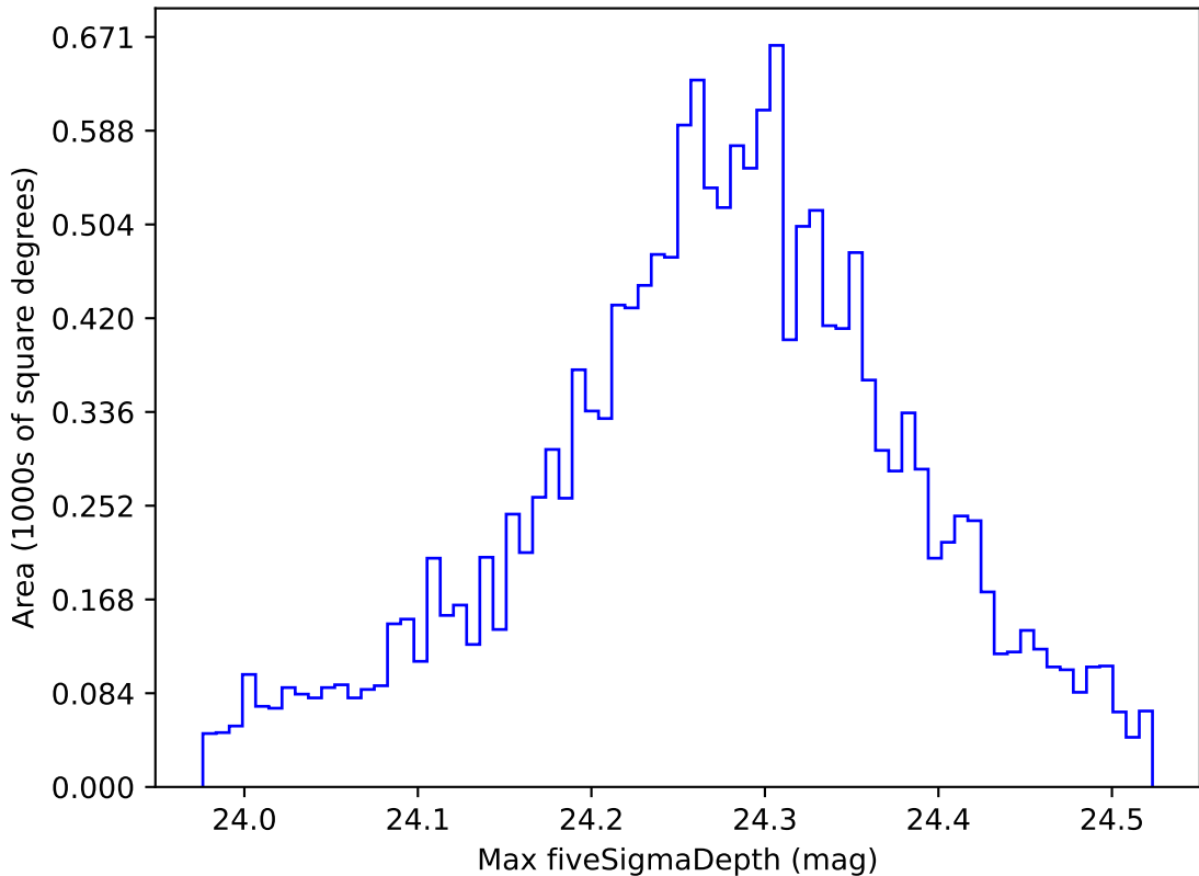
too_elab_r64_d2_griz_v3.4_10yrs WFD i band: Max fiveSigmaDepth
