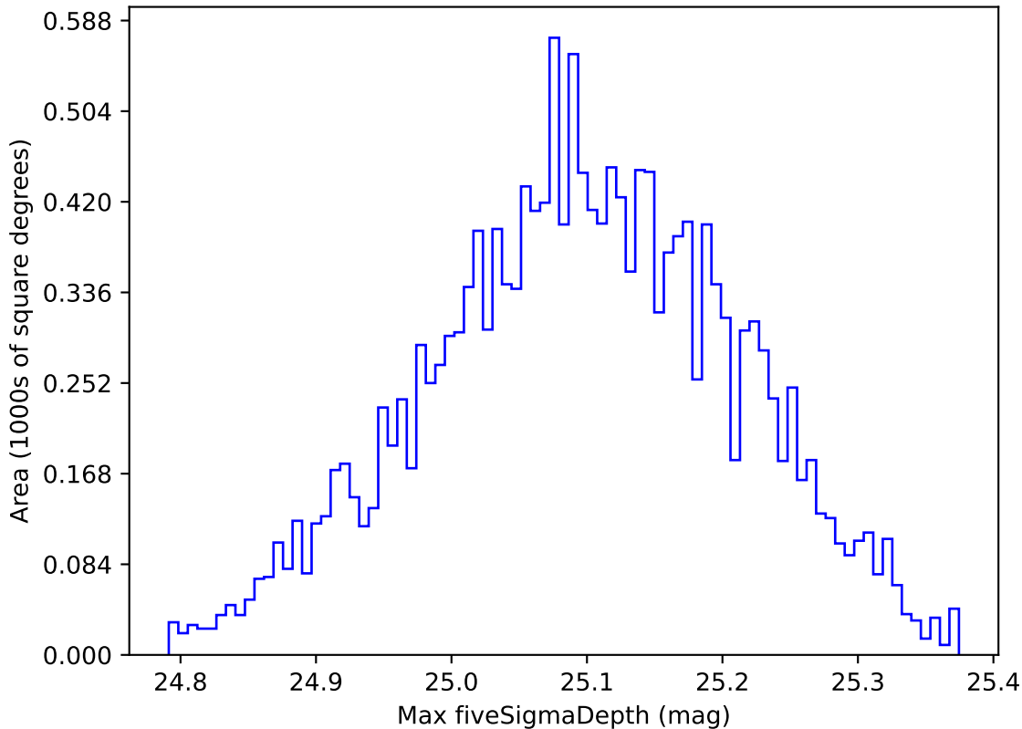
too_elab_r64_d2_griz_v3.4_10yrs WFD g band: Max fiveSigmaDepth
