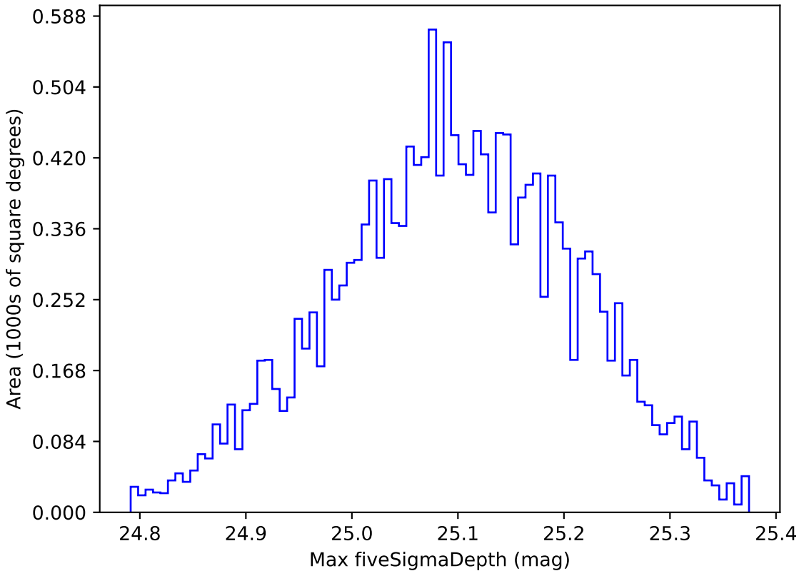
too_elab_r64_d2_griz_v3.4_10yrs WFD all bands: Max fiveSigmaDepth
