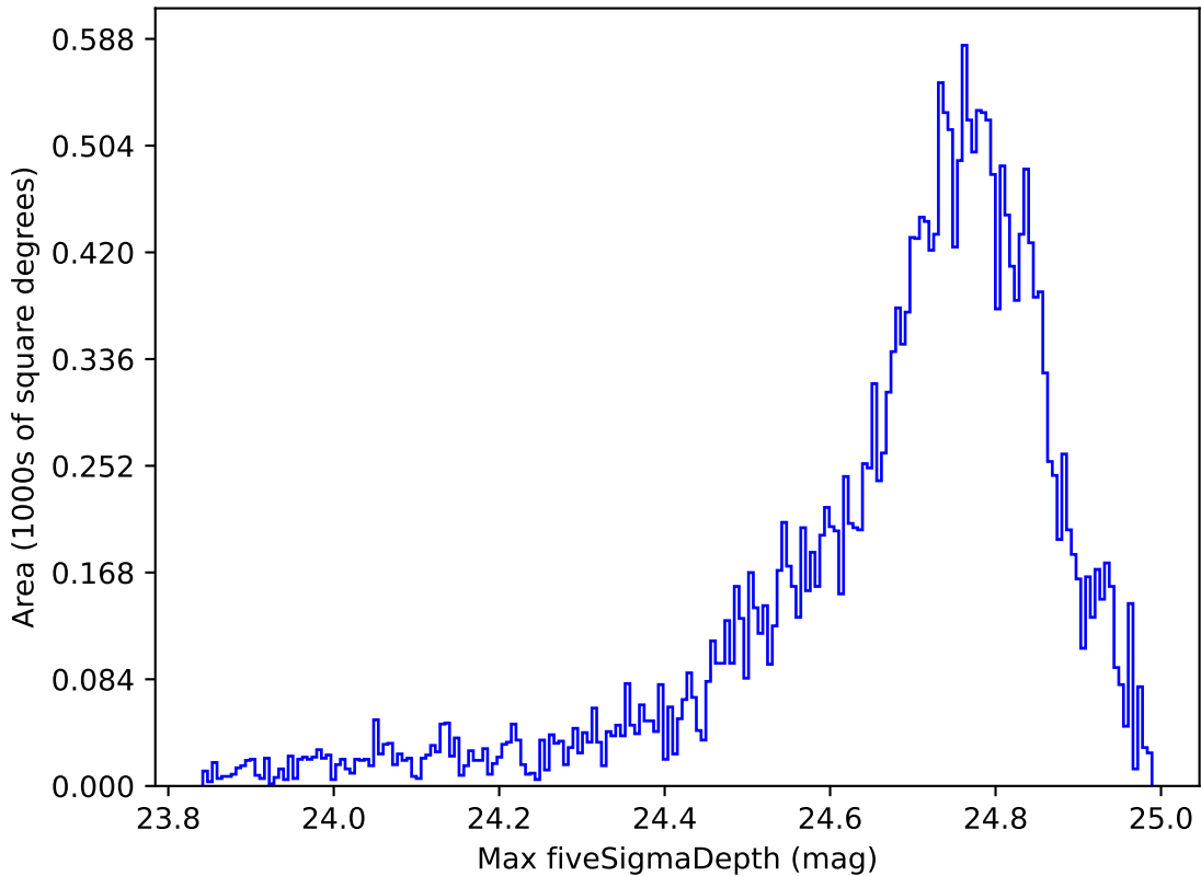
too_elab_r64_d2_griz_v3.4_10yrs All sky r band: Max fiveSigmaDepth
