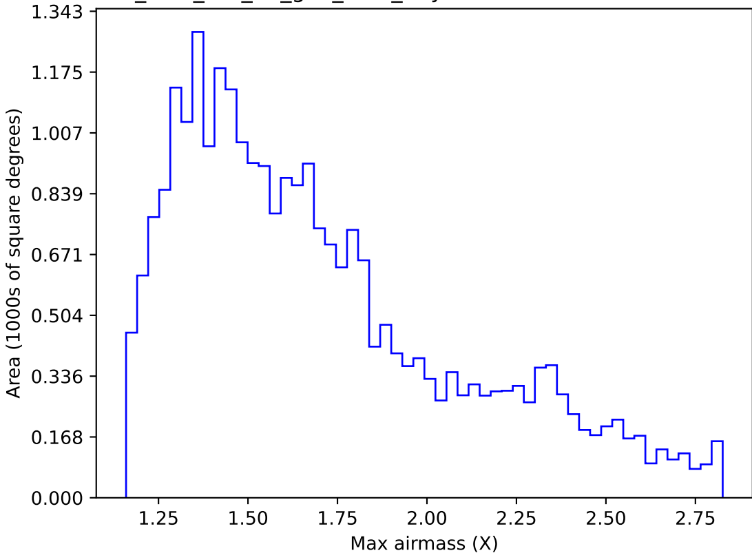
too_elab_r64_d2_griz_v3.4_10yrs Yr 1 z band: Max airmass
