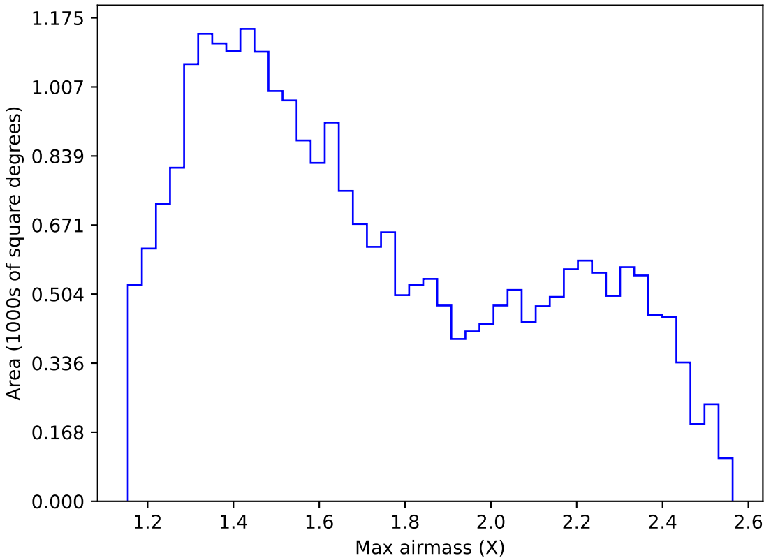
too_elab_r64_d2_griz_v3.4_10yrs Yr 1 r band: Max airmass
