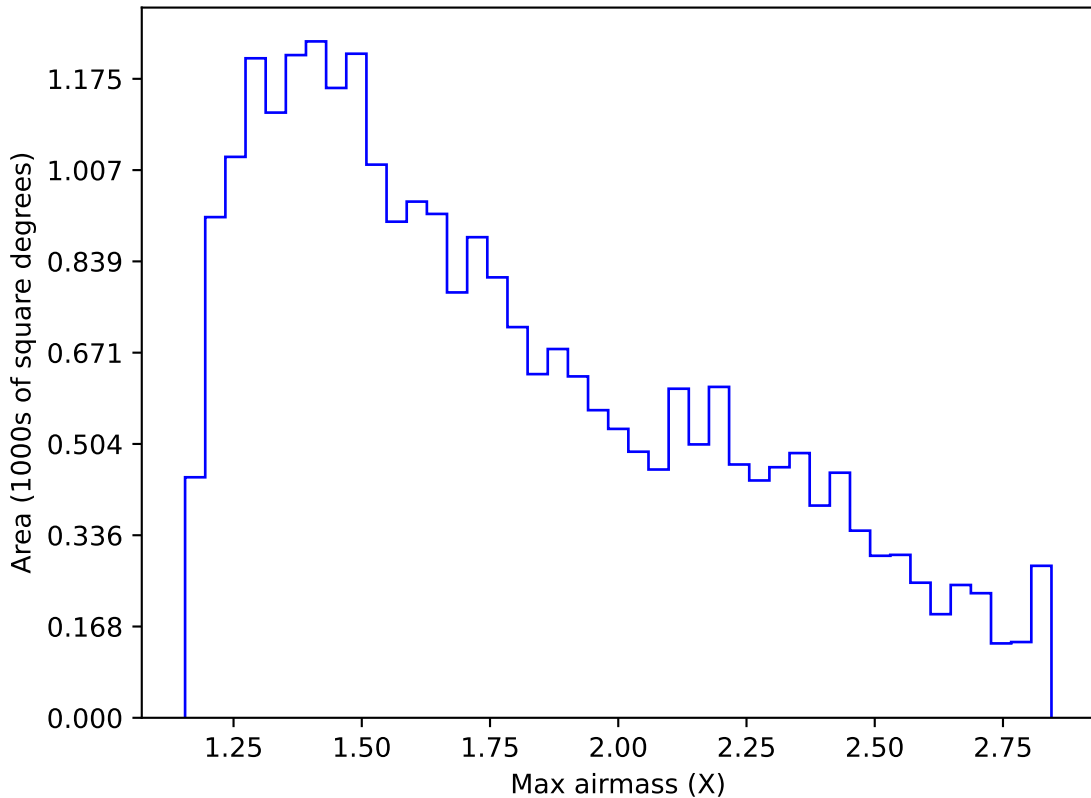
too_elab_r64_d2_griz_v3.4_10yrs Yr 1 i band: Max airmass
