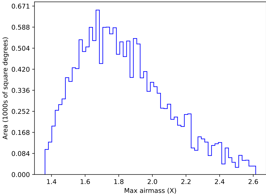
too_elab_r64_d2_griz_v3.4_10yrs WFD u band: Max airmass
