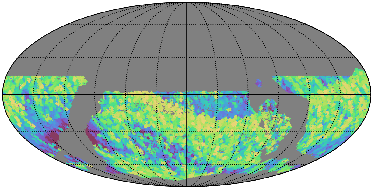
too_elab_r64_d2_griz_v3.4_10yrs WFD all bands: Max airmass
