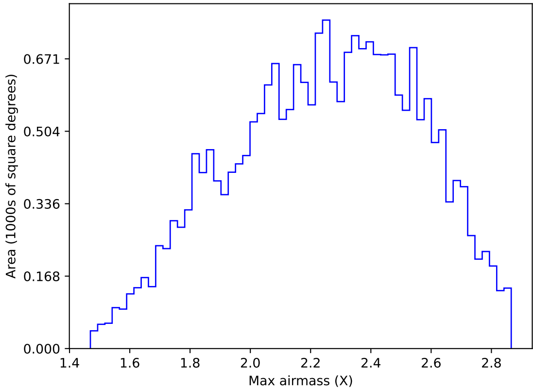
too_elab_r64_d2_griz_v3.4_10yrs All sky y band: Max airmass
