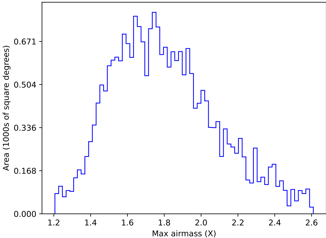
too_elab_r64_d2_griz_v3.4_10yrs All sky u band: Max airmass
