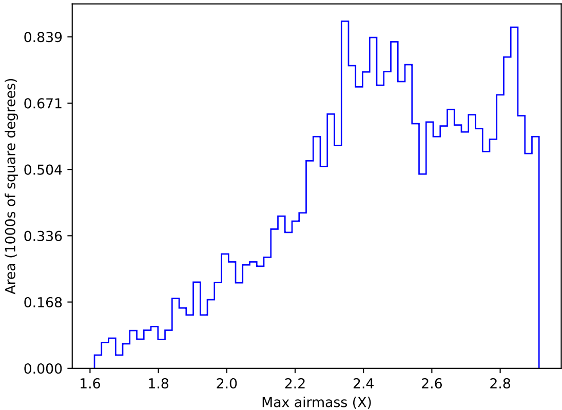
too_elab_r64_d2_griz_v3.4_10yrs All sky i band: Max airmass
