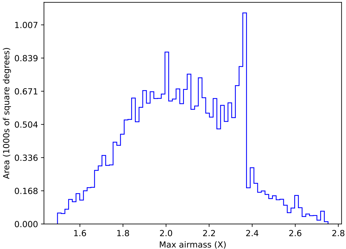
too_elab_r64_d2_griz_v3.4_10yrs All sky g band: Max airmass
