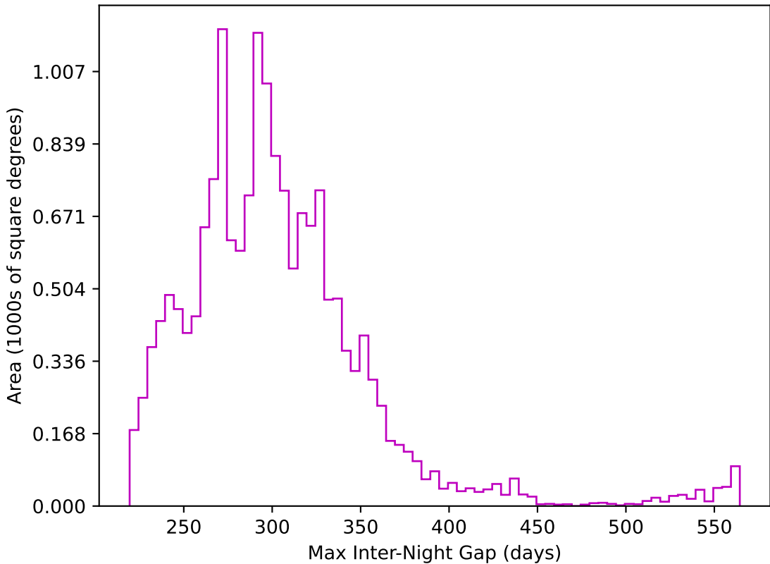
too_elab_r64_d2_griz_v3.4_10yrs WFD z band: Max Inter-Night Gap
