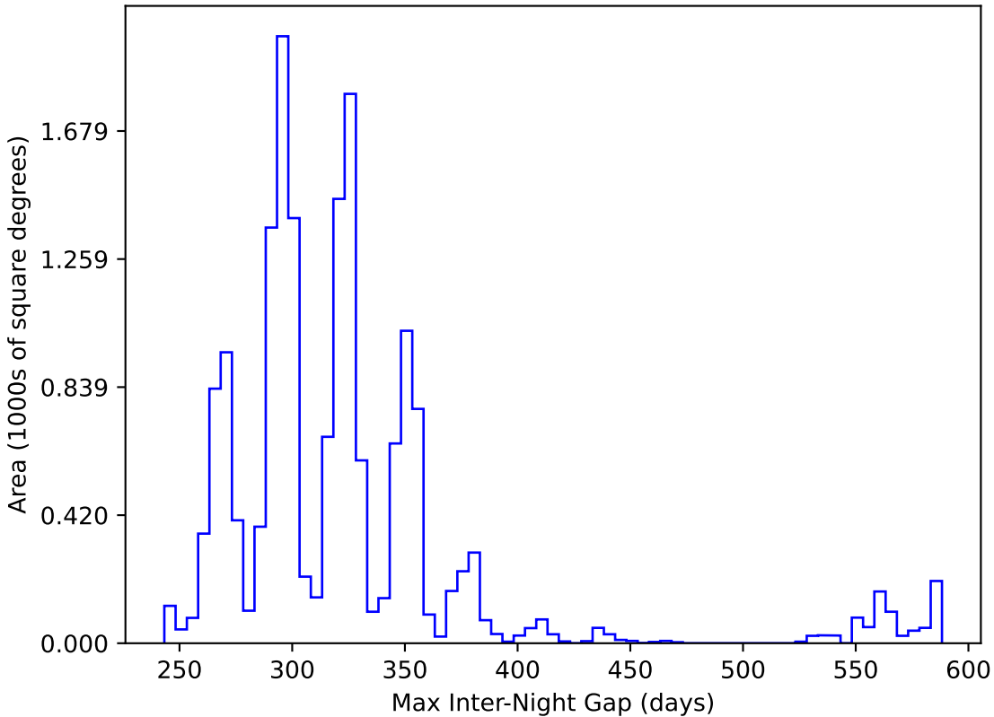
too_elab_r64_d2_griz_v3.4_10yrs WFD y band: Max Inter-Night Gap
