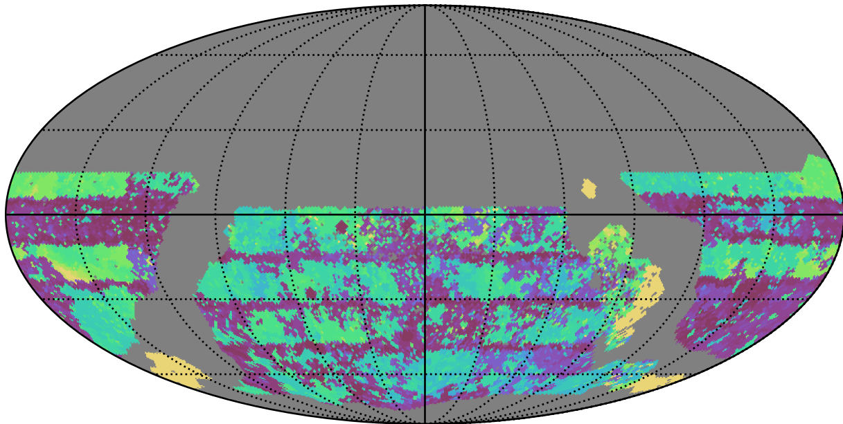
too_elab_r64_d2_griz_v3.4_10yrs WFD u band: Max Inter-Night Gap
