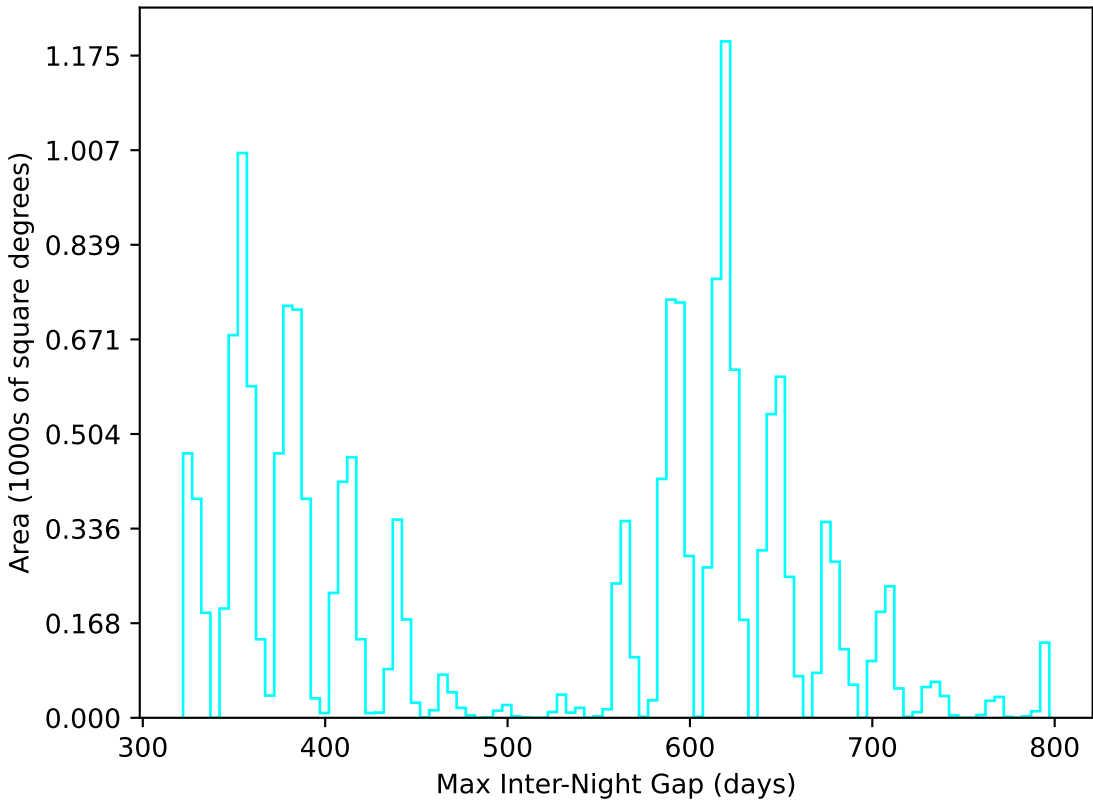
too_elab_r64_d2_griz_v3.4_10yrs WFD u band: Max Inter-Night Gap
