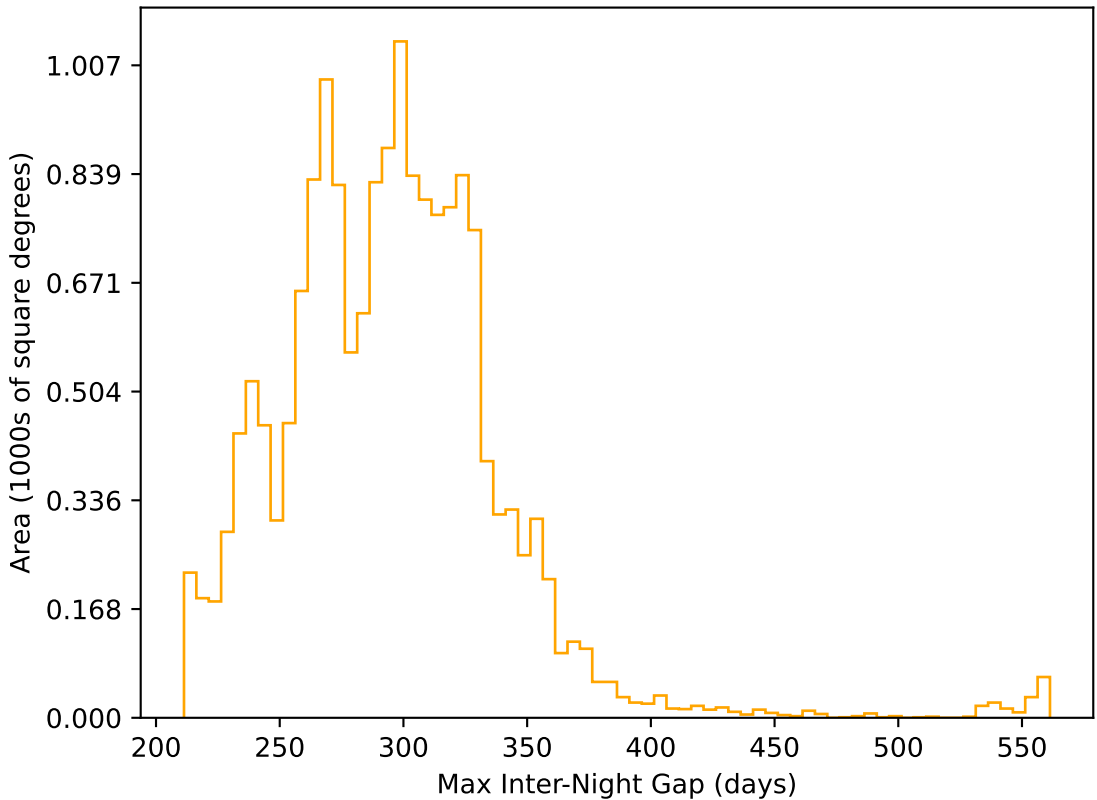
too_elab_r64_d2_griz_v3.4_10yrs WFD r band: Max Inter-Night Gap
