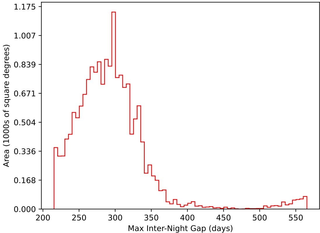
too_elab_r64_d2_griz_v3.4_10yrs WFD i band: Max Inter-Night Gap
