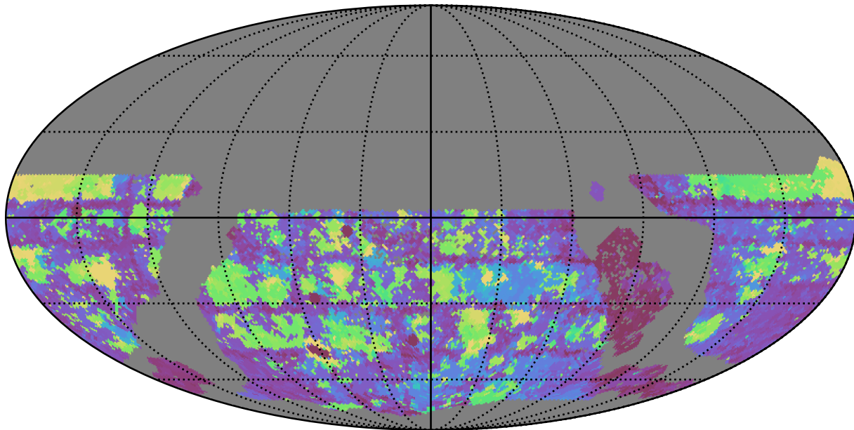
too_elab_r64_d2_griz_v3.4_10yrs WFD g band: Max Inter-Night Gap
