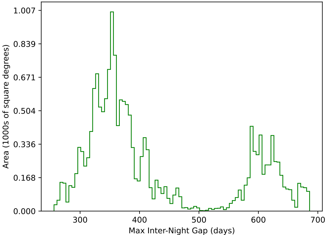
too_elab_r64_d2_griz_v3.4_10yrs WFD g band: Max Inter-Night Gap
