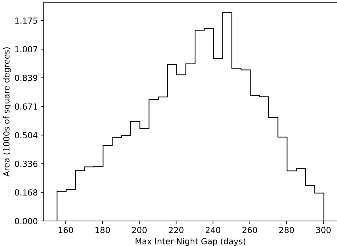
too_elab_r64_d2_griz_v3.4_10yrs WFD all bands: Max Inter-Night Gap
